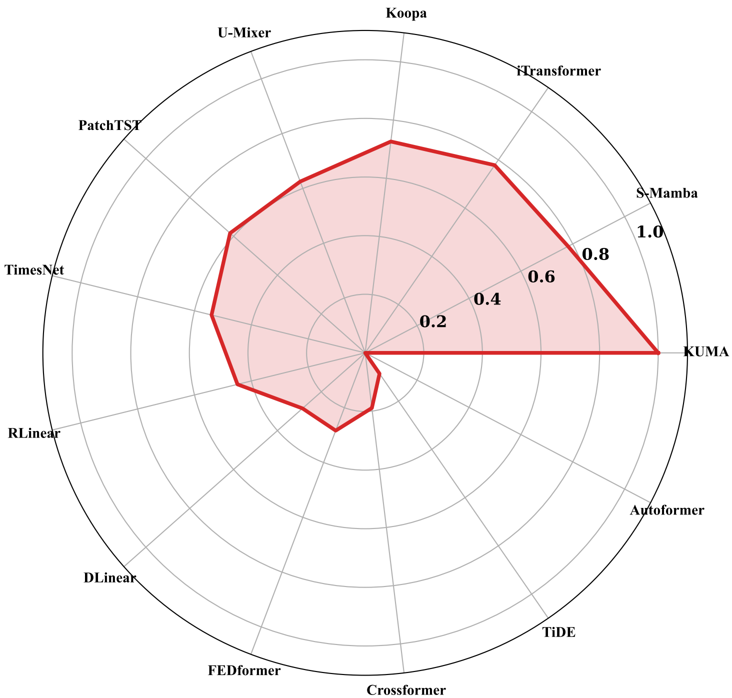
Radar Chart Based on Average Rank
